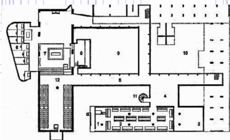
Refectory floor 1 Pantry, 2 Refectory, 3 Chapter-room, 4 Atrium, 5 Cloister, 6 Lower church, 7 High altar, 8 Sacristy, 9, 10 Courtyard, 11 Spiral staircase.
